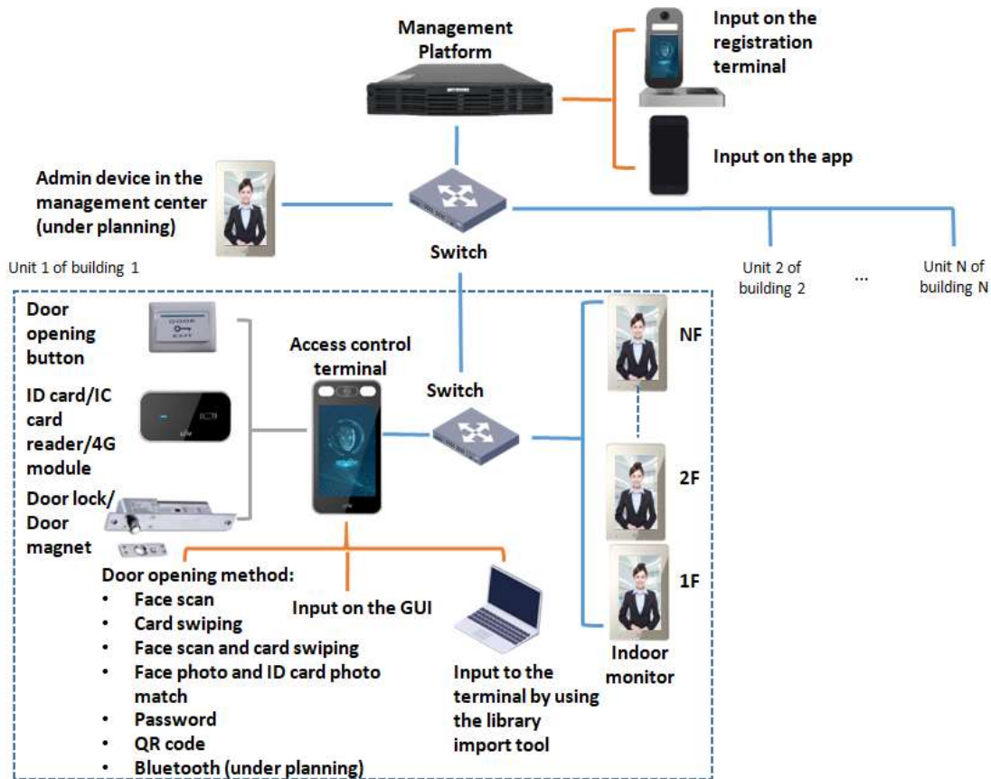
Figure2-1 Typical Network Topology
