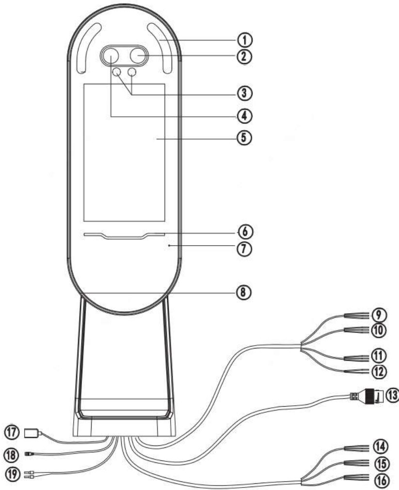
Figure3-3 Device Structure
