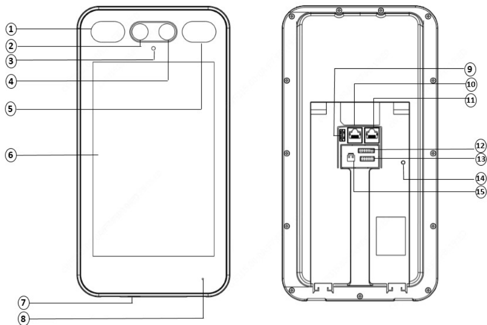
Figure3-1 Device Structure
