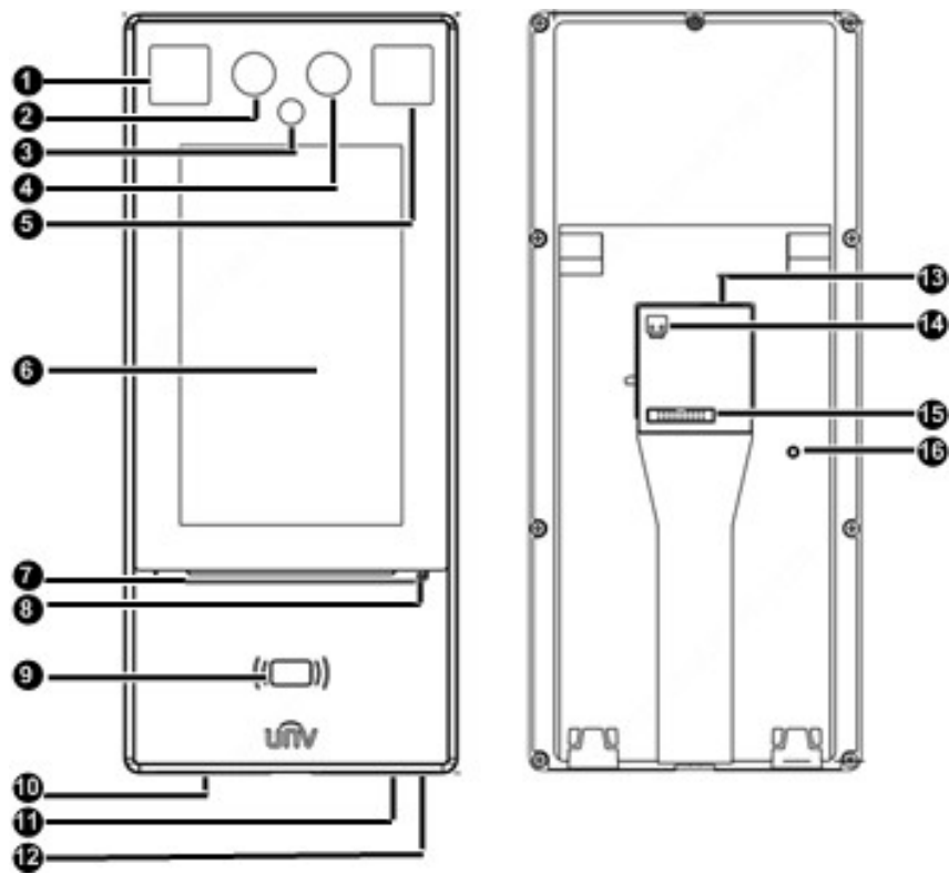
Figure3-2 Device Structure
